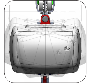
TROLLEY DESIGN - 15° TILT
