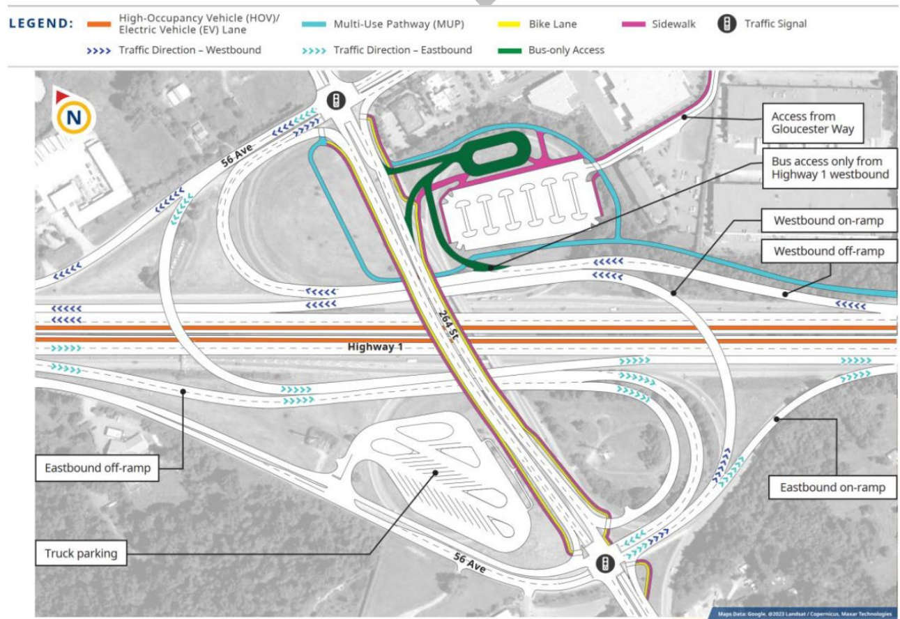
FIGURE 2 – 264 TH STREET INTERCHANGE CONCEPT
